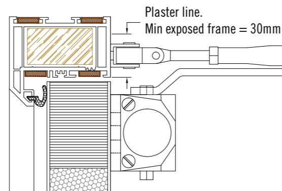
Overhead Closer detail PVCu frame
